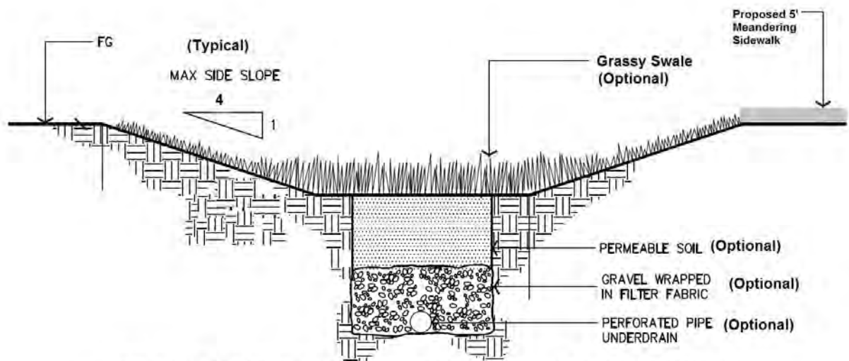
TYPICAL CROSS SECTION OF BIORETENTION GRASSY SWALE WITH UNDER DRAIN
