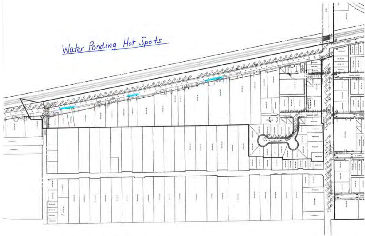
Figure 17B: Areas of Ponding Water after Major Rain Events (Hot Spots) Areas South of Yosemite Blvd (Phase 1B)
