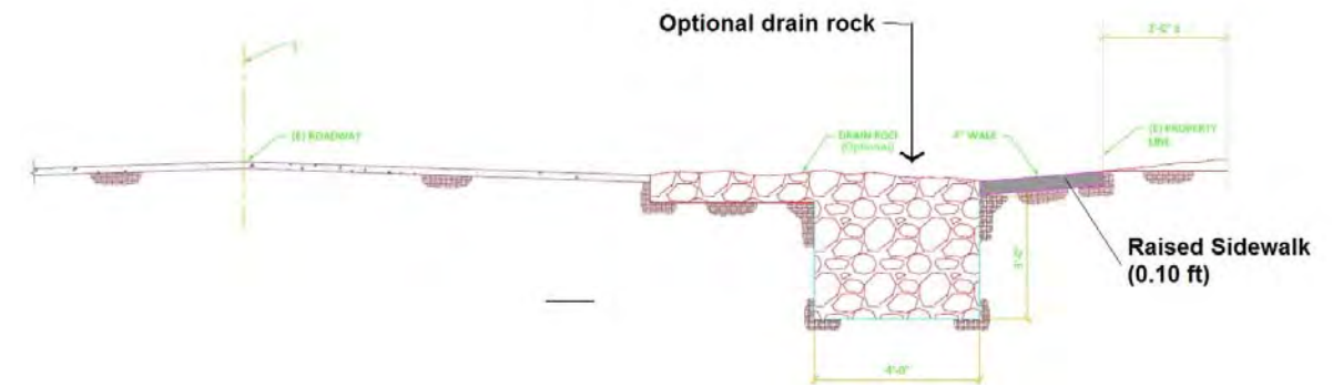
Figure 20: Bioretention Swale Cross Section with optional landscape and under drain
