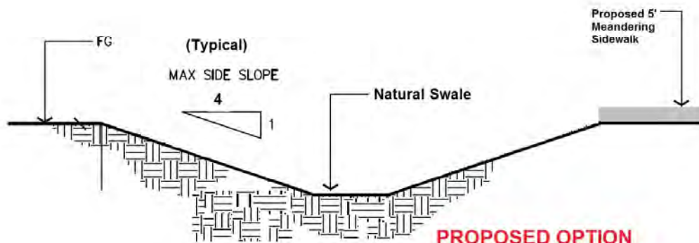
TYPICAL CROSS SECTION OF BIORETENTION SWALE WITH NO UNDER DRAIN
