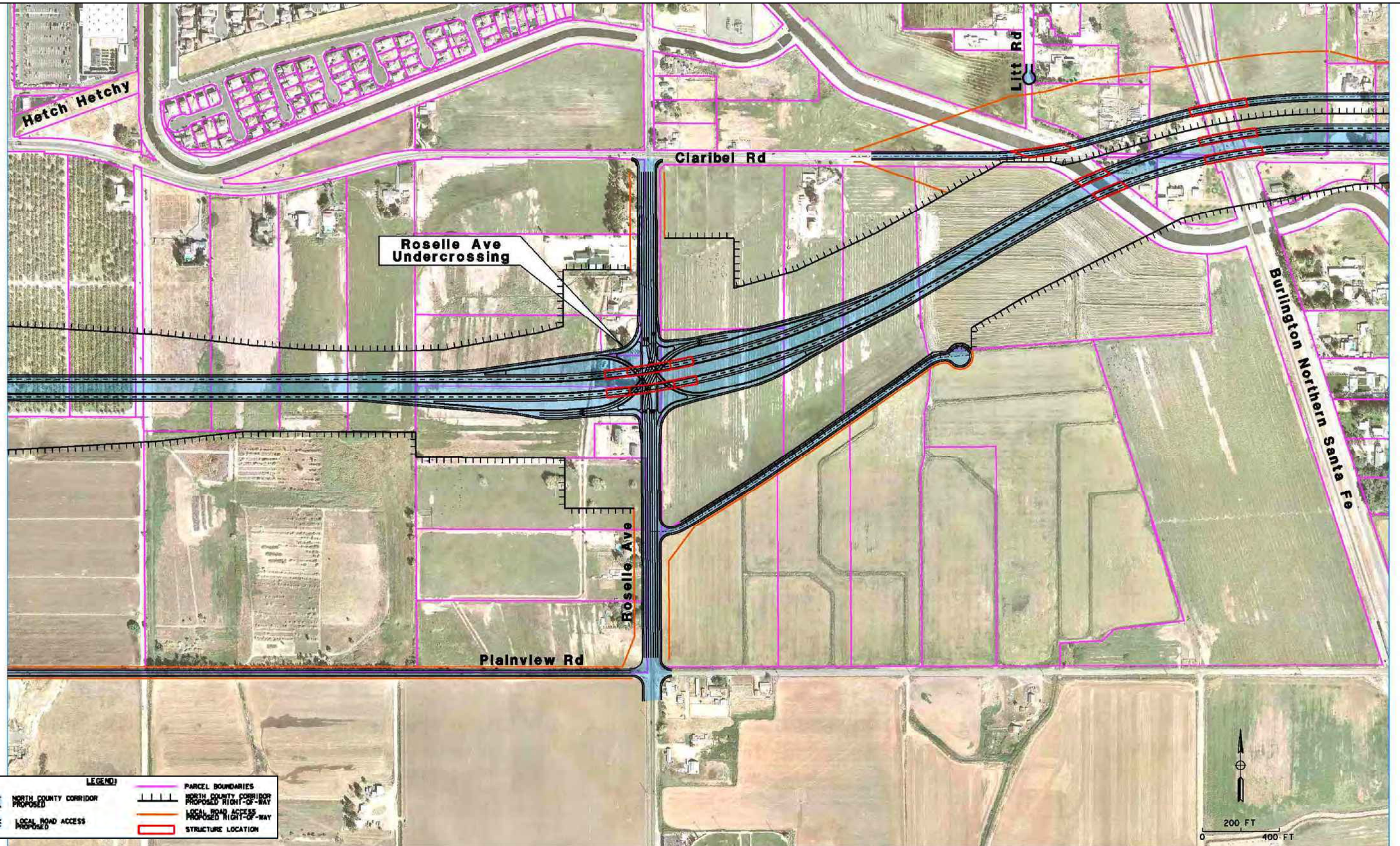
FIGURE 2.3.1-2 Example Single-Point Interchange EA: 10-0S8000, Project ID # 1000000263 North County Corridor New State Route 108 Project Stanislaus County, California
