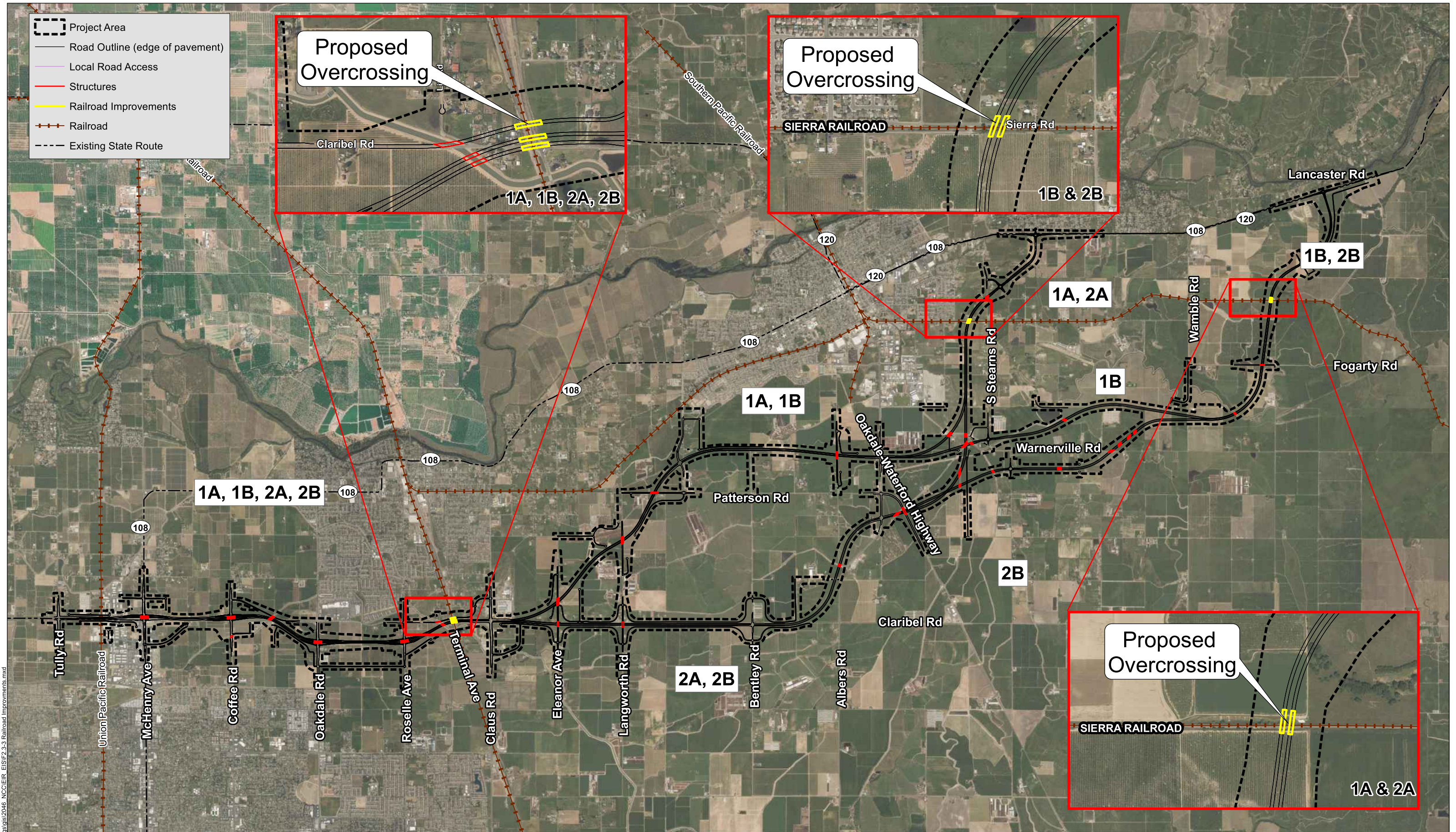
FIGURE 2.3.1-3 Railroad Improvements and Change EA: 10-0S8000, Project ID # 1000000263 North County Corridor New State Route 108 Project Stanislaus County, California
