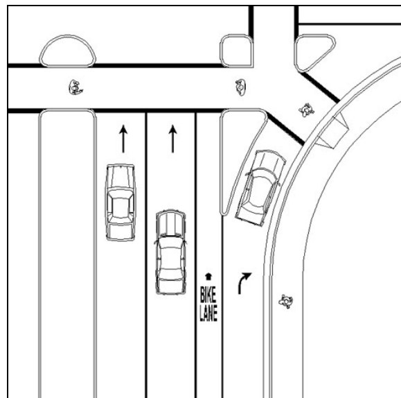
Figure B-27: Slip Turn Crossing Treatment
