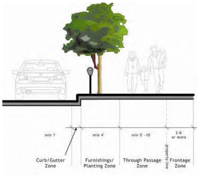
Figure B-1: Sidewalk Zones
