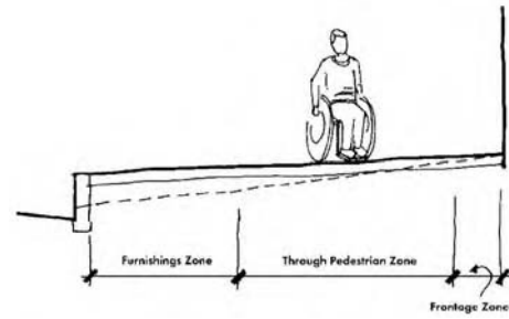
Figure B-12: Cross Slope
