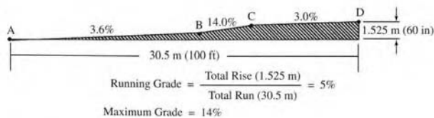
Figure B-11: Running Grade and Maximum Grade
