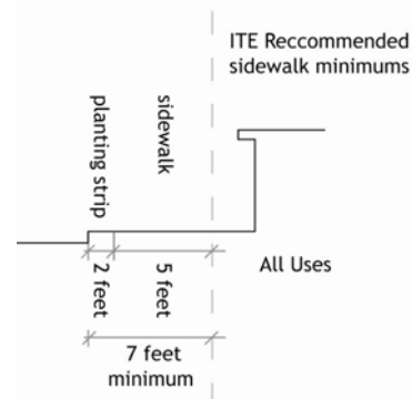
Figure B-2: Sidewalk Minimums
