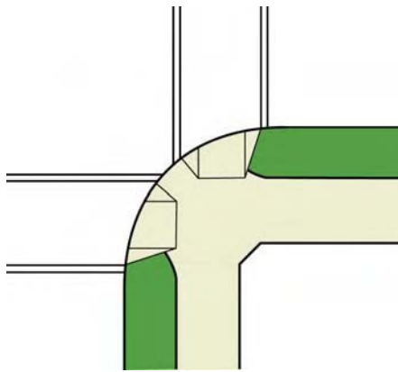
Figure B-31: Perpendicular Curb Ramp Design
