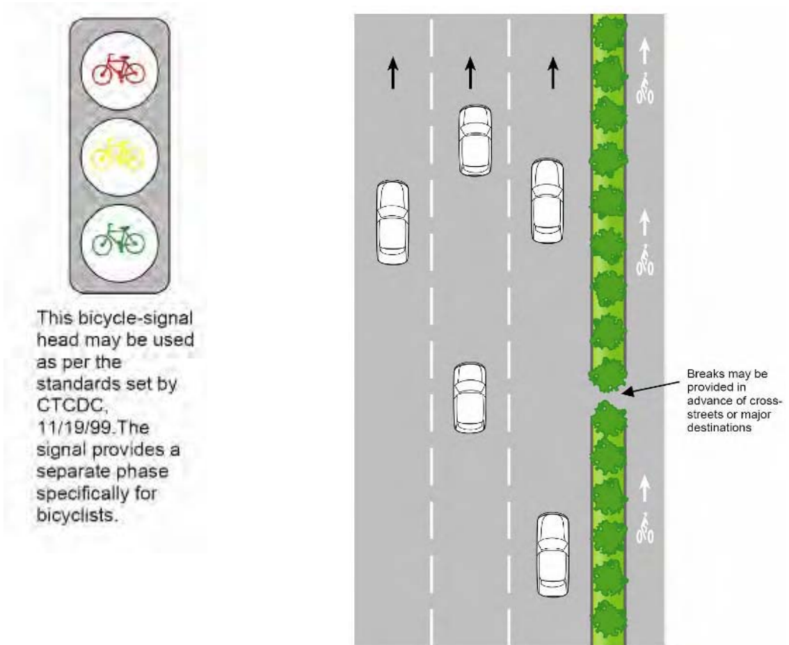
Figure A-3: One-way Bike Path (Cycle Track) and Bicycle Signal Head
