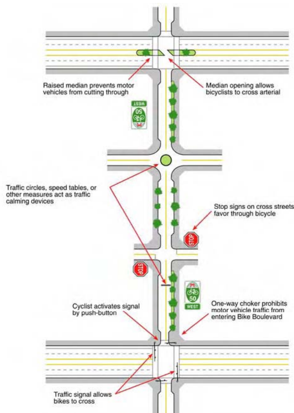
Figure A-13: Example Bicycle Boulevard
