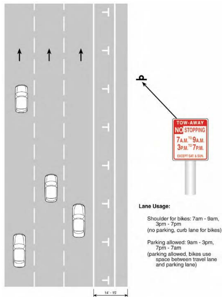
Figure A-8: Floating Bicycle Lane
