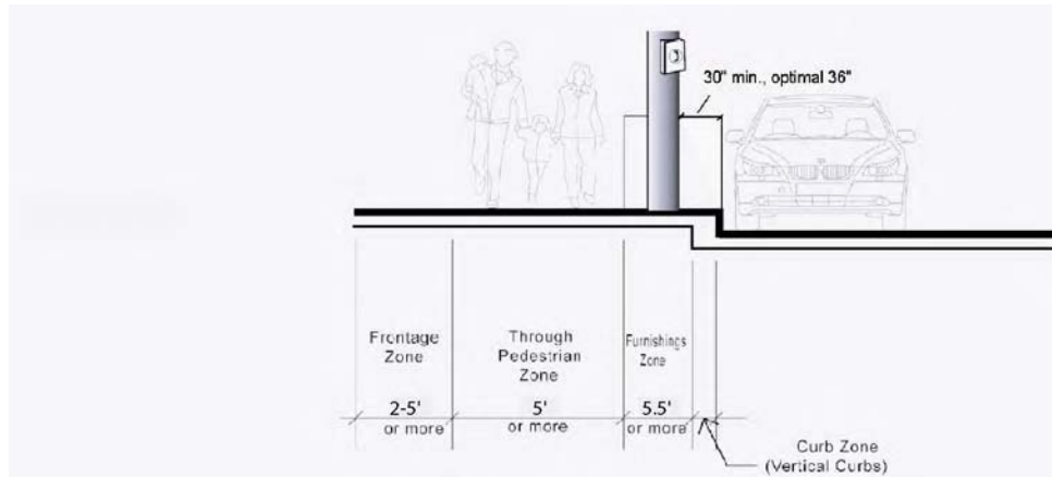
Figure B-9: Utility Poles and Structure Placement
