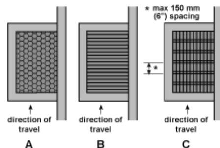
Figure A-5: Examples of bicycle friendly drainage grates
