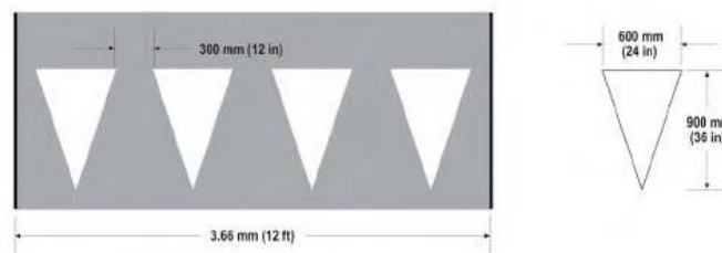
Figure B-23: Yield Line Specifications
