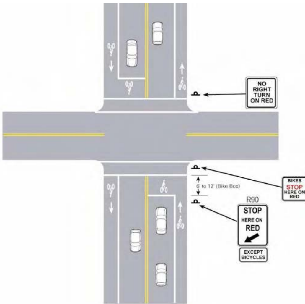
Figure A-9: Bicycle Box
