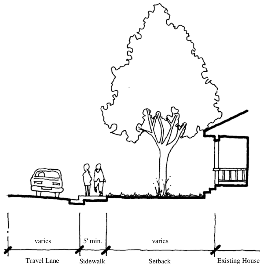
Figure B-3: Sidewalks on Narrow Streets
