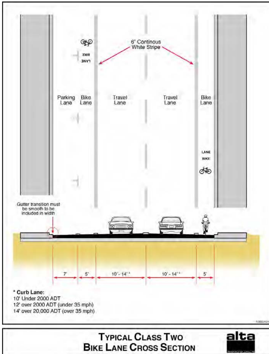
Figure A-4: Typical Class II Facility Cross-Section
