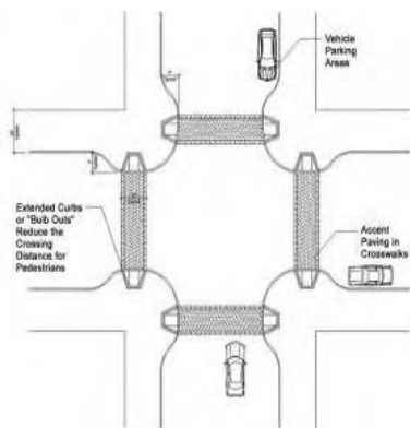
Figure B-26: Curb Extensions
