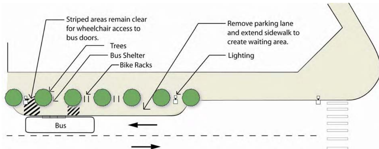
Figure B-17: Accessible Bus Bulb Out
