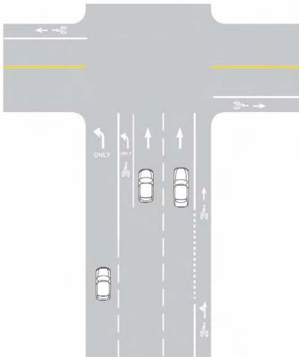
Figure A-10: Bicycle Left-turn Pocket Lane
