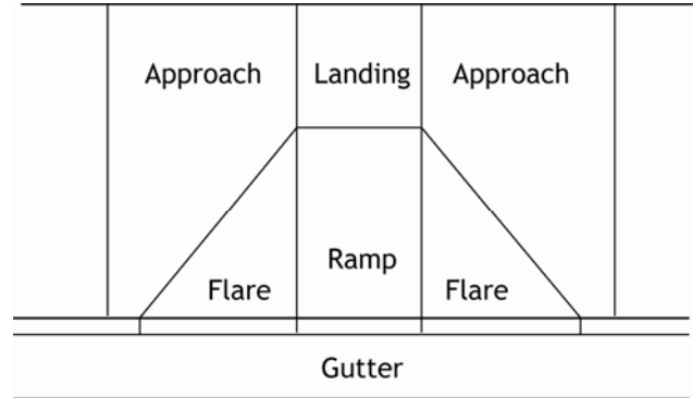
Figure B-30: Curb Ramp Components
