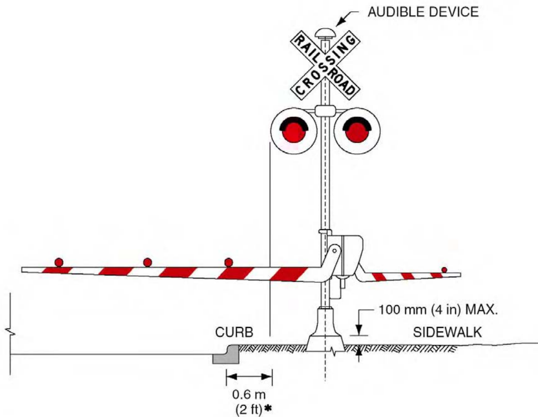
Figure B-14: Railroad Arm on Sidewalk
