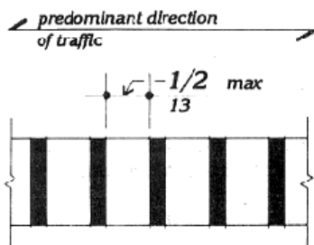
Figure C-7: Ventilation Grates
