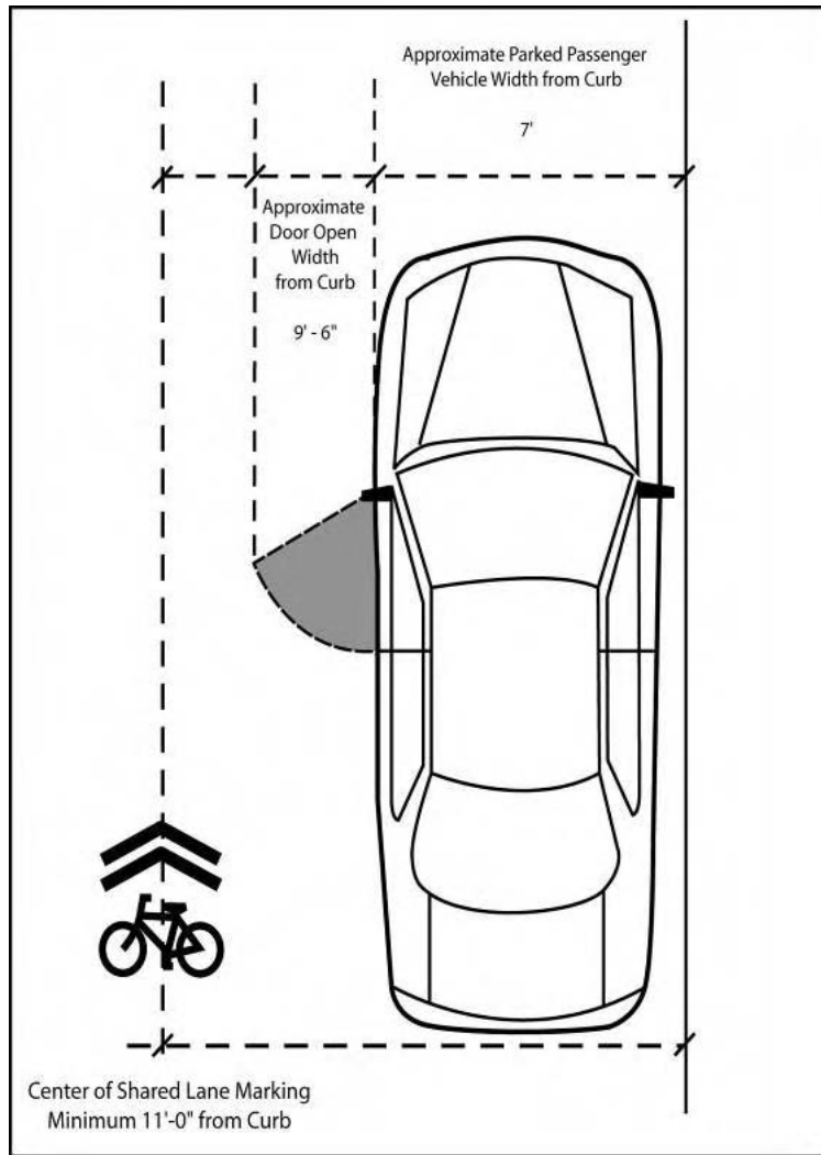
Figure A-11: Shared Lane Marking Placement
