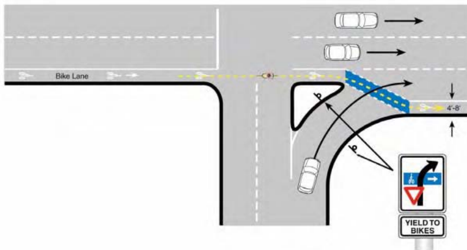
Figure A-6: Colored Bicycle Lane Through Conflict Zone
