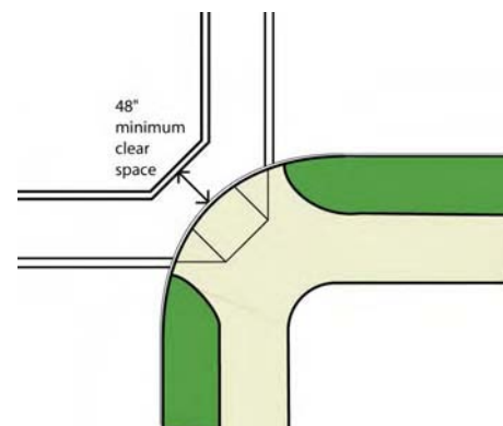
Figure B-32: Diagonal Curb Ramp Design
