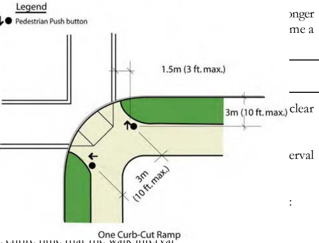
Figure B-29: Recommended Pushbutton Locations
