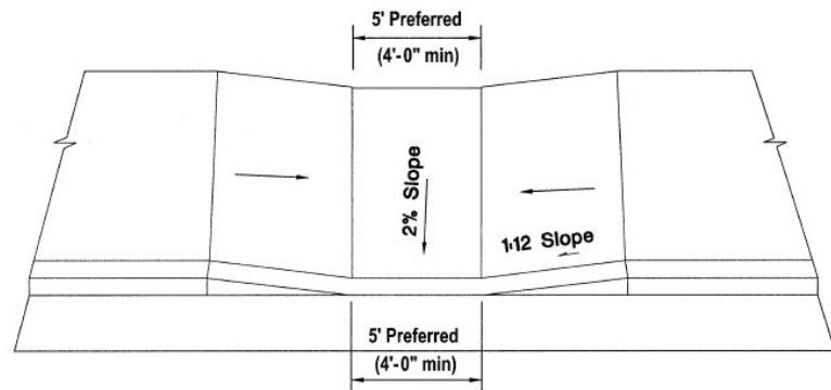
Figure B-33: Parallel Curb Ramp Design
