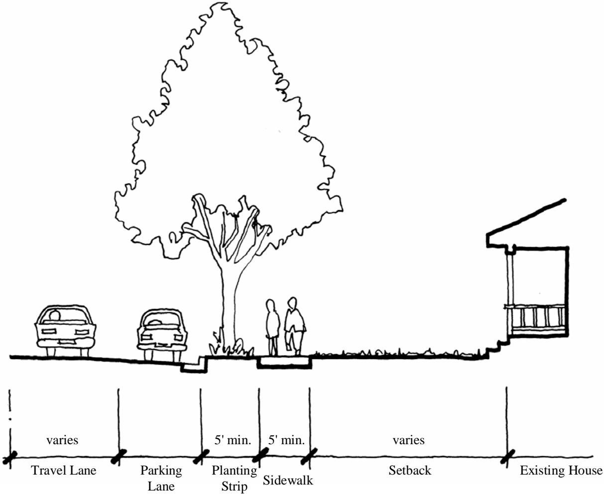
Figure B-5: Sidewalk with Planting Strip
